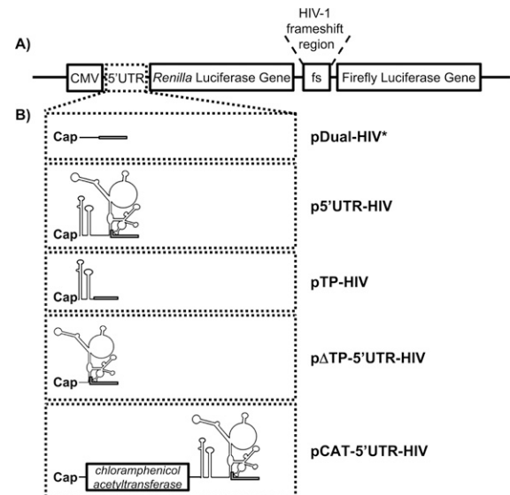
FIGURE 2. Scheme of the vectors used to assess HIV-1 frameshift efficiency. (A) Representation of a dual-luciferase reporter. All of the reporters used in this study are derivatives of this dual-luciferase reporter, which differ in their 5' UTR. They contain the Renilla (Rluc) and the firefly luciferase (Fluc) coding sequences, under control of a CMV promoter, and separated by the HIV-1 frameshift region (nucleotides 1608–1685 in pLAI). Rluc is synthesized by all of the ribosomes translating the mRNA, whereas Fluc is synthesized, as a fusion to Rluc, only by ribosomes that make a -1 frameshift in the frameshift region. (B) Details on the 5' UTR of the different reporter mRNAs used in this study. Plasmid pDual-HIV* has a short and unstructured 5' UTR. The plasmid p5'UTR-HIV contains the complete 5' UTR of HIV-1 full-length mRNA (nucleotides 1–335 in pLAI). The plasmid pTP-HIV contains the beginning of the 5' UTR of HIV-1 full-length mRNA encompassing the TAR and poly(A) structures (nucleotides 1–106 in pLAI). The plasmid pΔTP-5'UTR-HIV contains a part of the HIV-1 full-length mRNA 5' UTR (nucleotides 95–335 in pLAI), which encompasses HIV-1 IRES but not TAR and poly(A). Finally, the plasmid pCAT-5'UTR-HIV was designed such that translation of the CAT sequence results from a cap-dependent initiation, whereas the production of the luciferases, preceded by the 5' UTR of HIV-1 full-length mRNA, results from an IRES-dependent initiation. In pDual-HIV* and pTP-HIV, only the cap-dependent initiation is available. In pΔTP-5'UTR-HIV and p5'UTR-HIV, both cap- and IRES-dependent initiations could be possible. In all of the plasmids, the AUG initiator codon for Rluc is followed by the first 30 nt from the gag coding region. Also, an oligonucleotide coding for a peptide linker was inserted between the nucleotide from gag and the beginning of the Rluc coding sequence. The AUG codon and the 30 nt from gag plus the linker are represented by an open box.
